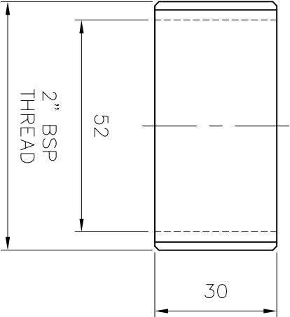
(SCALE-1:4) DETAIL-A BUSH FOR COUPLER
